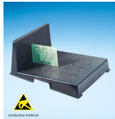
Art. No.: LP 1 printed boards L-Profil Dimensions: 200 x 274 x 93 Art. No.: LP 2 printed boards L-Profil Dimensions: 350 x 263 x 125 25 slots for printed boards transport/ storage service workshop
